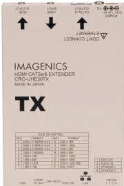
CRO-UHE30TX (送信器)
